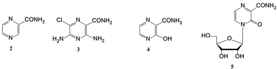
Fig. 3. Some structural analogs of favipiravir: 2 – 2-pyrazinecarboxamide; 3 – 3,5-diamino-6-chloro-2-pyrazinecarboxamide; 4 – 3-hydroxypyrazine-2-carboxamide (T-1105); 5 – 3-oxo-4-(β-D-ribofuranosyl)-2-pyrazinecarboxamide (T-1106)
