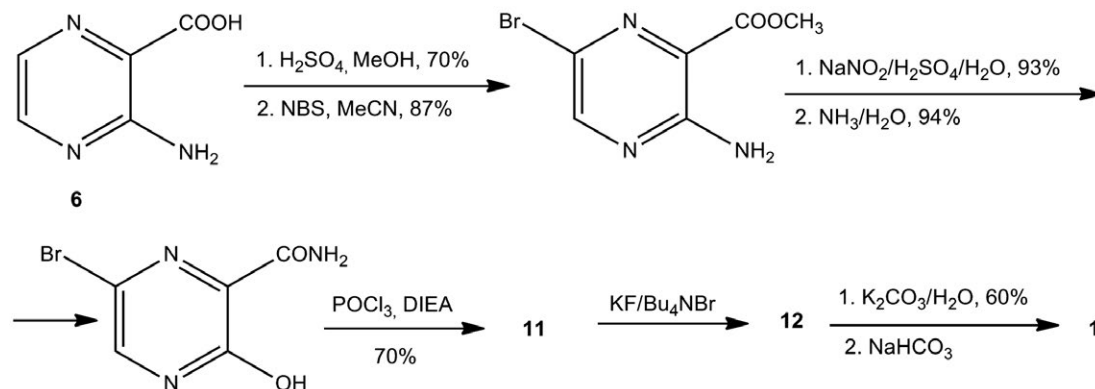
Fig. 8. Synthesis of favipiravir (1) according to the Liu Feng procedure
