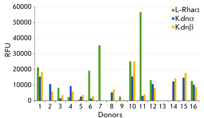
Fig. 3. Binding of human IgG-class serum antibodies (from 16 donors) to Kdn monosaccharide in its \alpha - and \beta -spacer form compared to \alpha L-rhamnose (L-Rha \alpha ). The sialic PGA (format #1) data are presented. The cutoff value was subtracted
