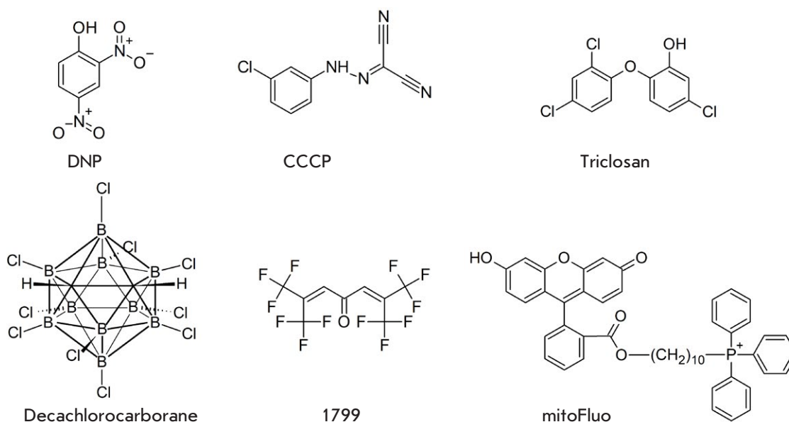
Fig. 1. Chemical structures of conventional protonophores (top row) and unconventional protonophores (bottom row). DNP – 2,4-dinitrophenol; CCCP – carbonyl cyanide-m-chlorophenyl hydrazone; triclosan – 2,2',4'-trichloro-2'-hydroxydiphenyl ether; decachlorocarborane; 1799 – \alpha, \alpha' -bis(hexafluoroacetyl)acetone; mitoFluo – a conjugate of fluorescein and the triphenylphosphonium cation
