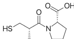
Fig. 1. Amino acid sequences of BPPs (A) and the structure of captopril (B). Z is a pyroglutamic acid residue
