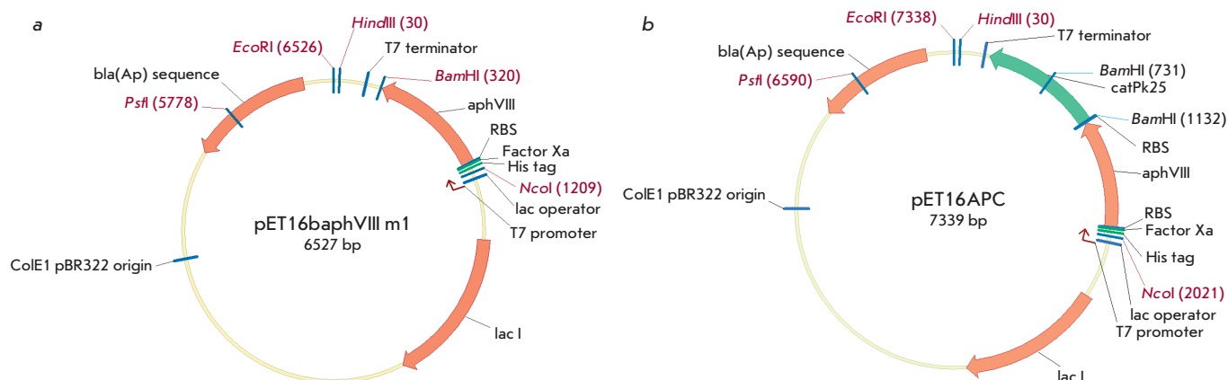
Fig 4. Vectors: a – pET16baphVIII m1 containing aphVIII mutant variants: aphVIII146-1 , aphVIII146-2 , aphVIII 146-3 , aphVIII146-4 and primary aphVIII146-S . b – pET16APC containing pk25 and aphVIII mutant variants aphVIII146-1 , aphVIII146-2 , aphVIII146-3 , and primary aphVIII146-S .
