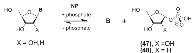
Scheme 4
