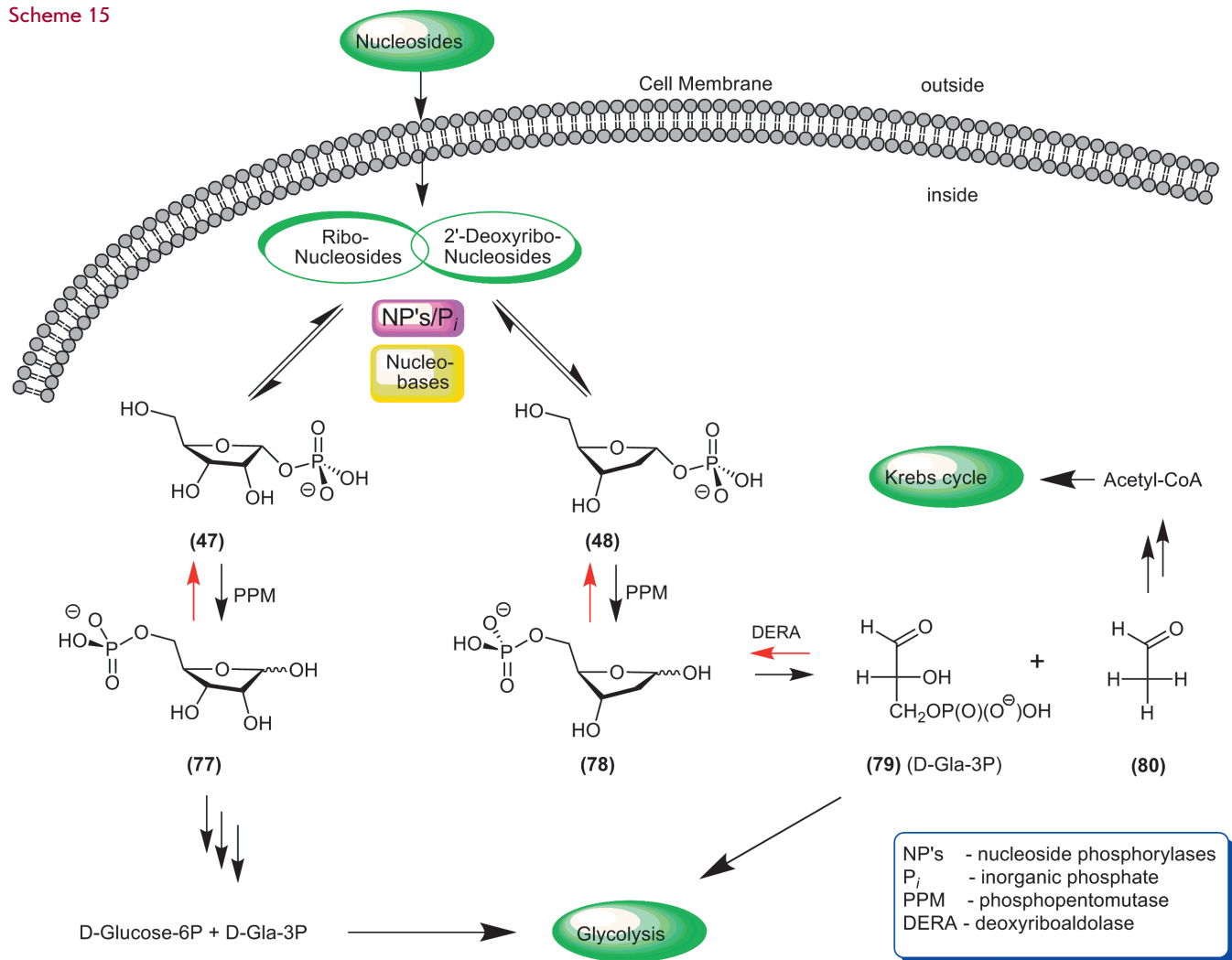
Scheme 15
