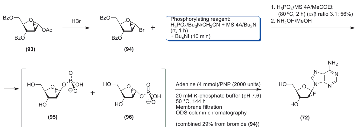
Scheme 21
