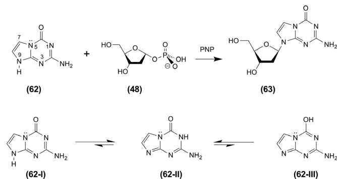
Scheme 10
