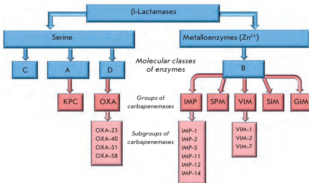
Fig. 2. Classification of carbapenemases into groups and subgroups based on the alignment of amino acid sequences and their correspondence to molecular classes of β-lactamases.
