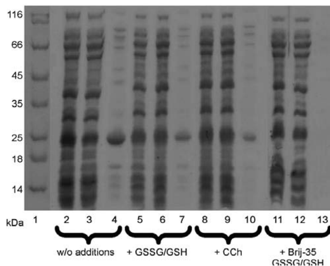
Fig. 2. Electrophoresis analysis of the cell-free synthesis of \alpha 7ED/C116S/DTES . 1- markers of molecular weights; 2, 5, 8, 11 – total protein fraction of translation mixture; 3, 6, 9, 12 – soluble protein fraction of translation mixture; 4, 7, 10, 13 - insoluble protein fraction of translation mixture.
